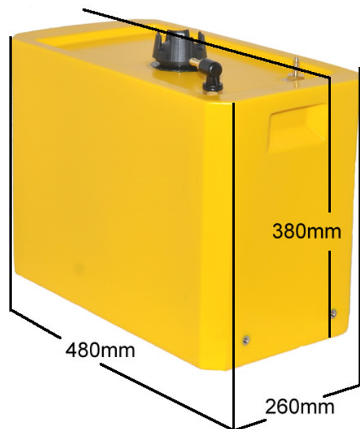
LA1995 - 35 Litre diesel - 38mm 90 degree with pick up LA1996 - 35 Litre tank - 38mm 90 deg with 5/16" outlet LA1997 - 35 Litre tank - 38mm 90 deg with 3/8" outlet
